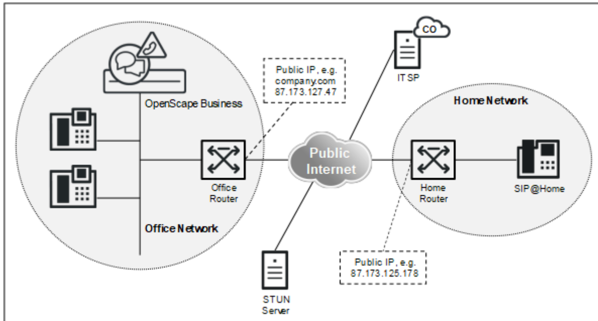
Figure 7: Device@Home (SIP Device@Home or System Device@Home) components
