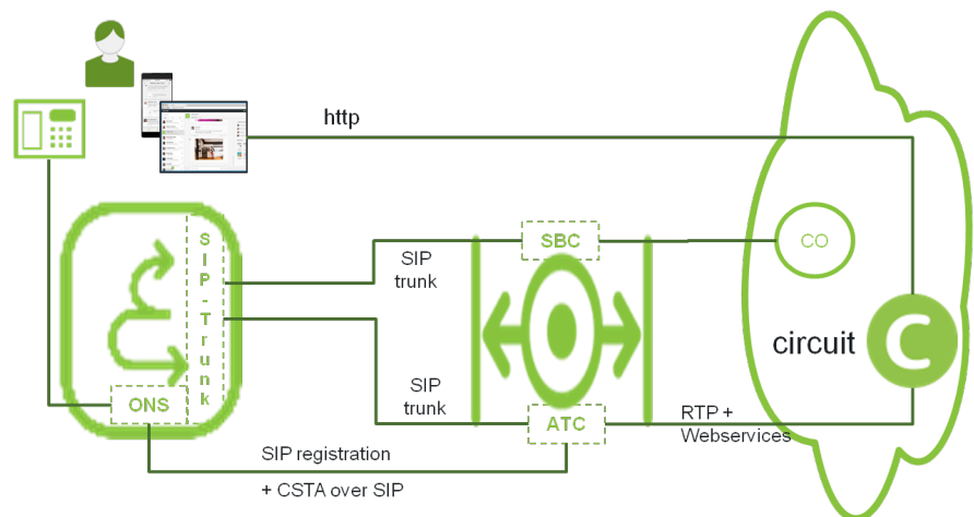
Figure 58: Advanced Telephony Connector (ATC)
