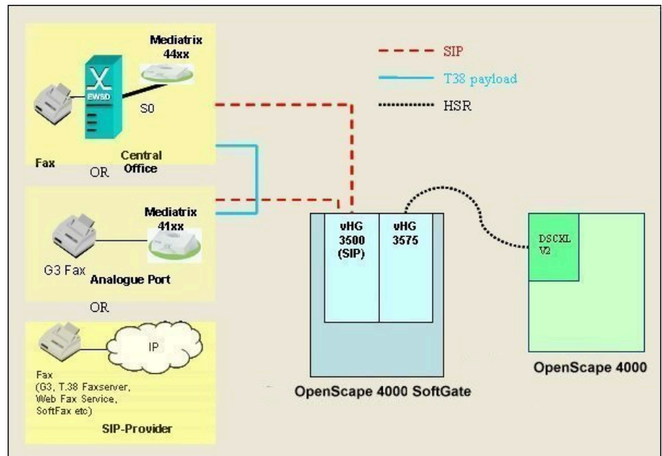
Figure 20: Fax between SIP Message Proxy enabled endpoints
