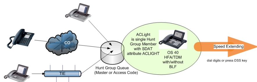
Figure 70: Attendant Light scenario
