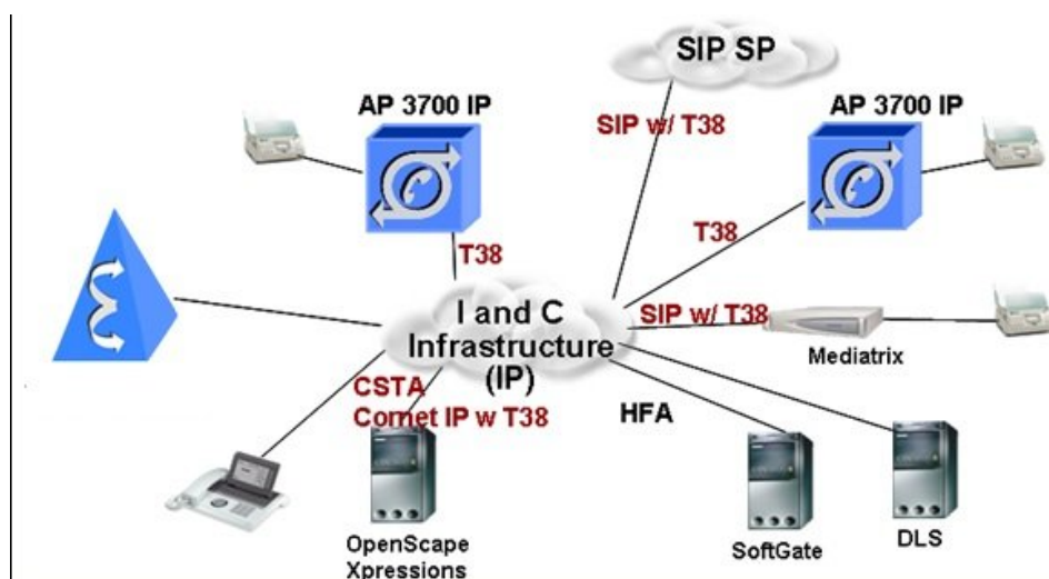
Figure 14: Overview T.38 support in OpenScape 4000 environment
