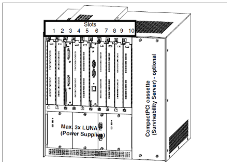
Figure 12: AP 3700IP front view
