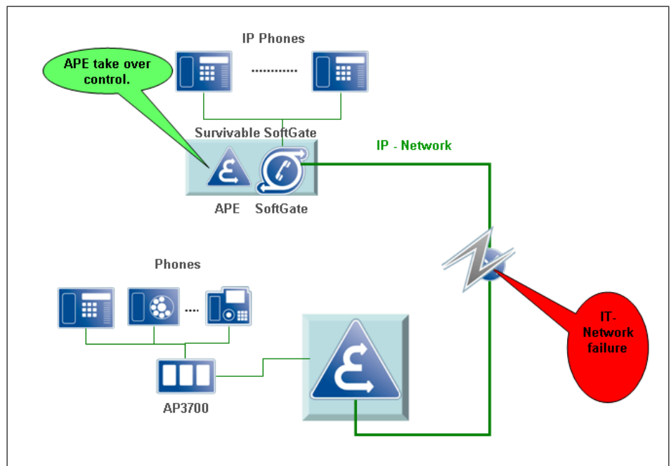
Figure 34: APE with Survivable OpenScape 4000 SoftGate
