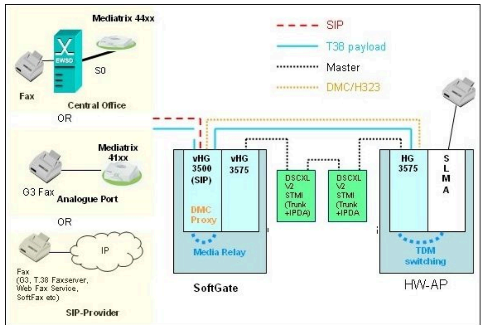
Figure 15: Media Relay Scenario with DMC
