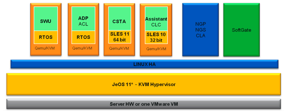
Figure 8: OpenScape 4000 Data Center Edition
