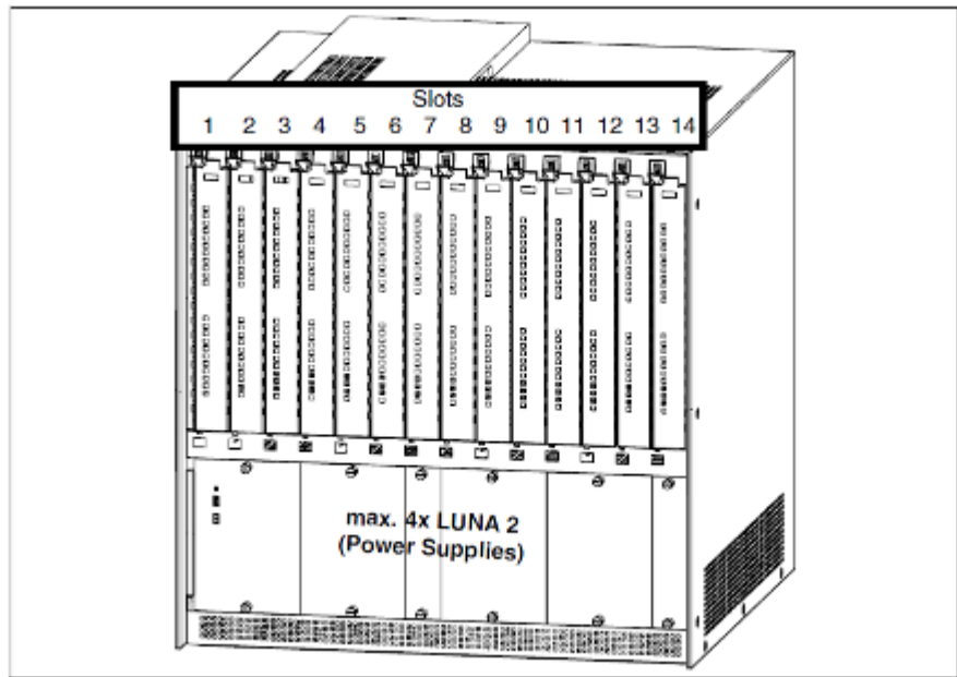
Figure 10: AP 3700 front view
