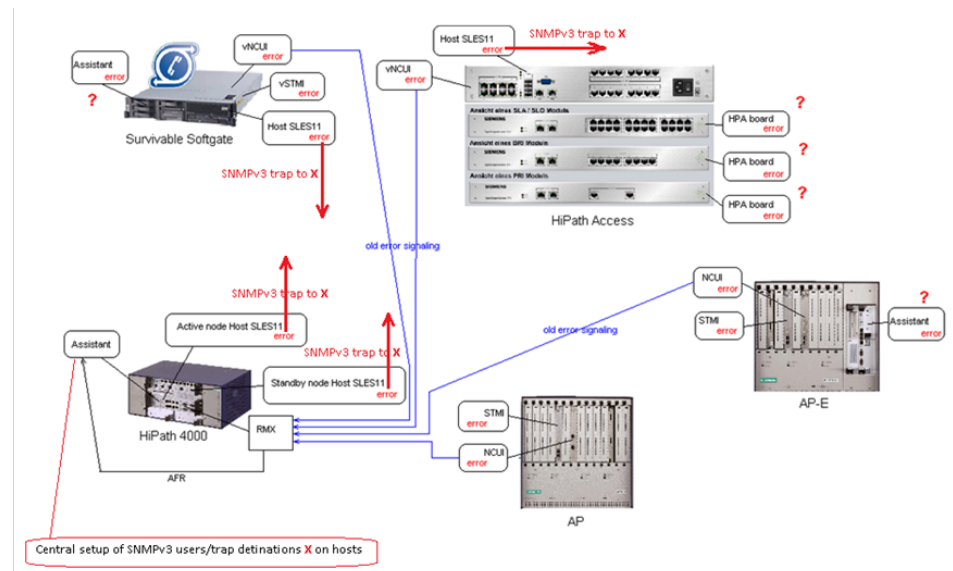
Figure 75: SNMP service
