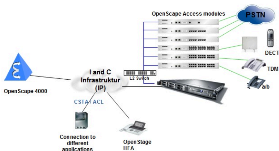
Figure 29: Scenario with OpenScape 4000 SoftGate
