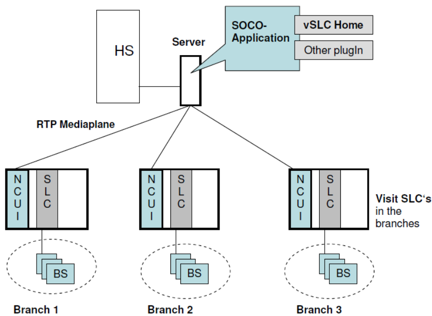
Figure 18: Virtual home SLC in an IPDA environment
