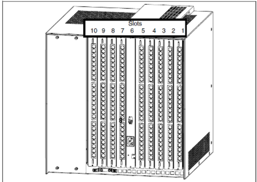
Figure 13: AP 3700IP back view with patch panels
