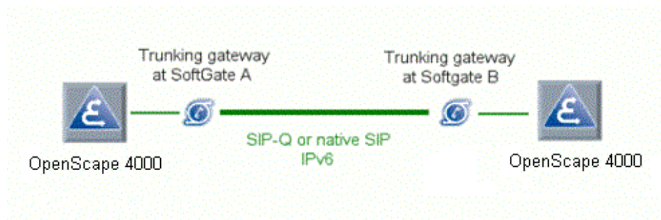
Figure 19: SIP-Q Trunking with IPv6
