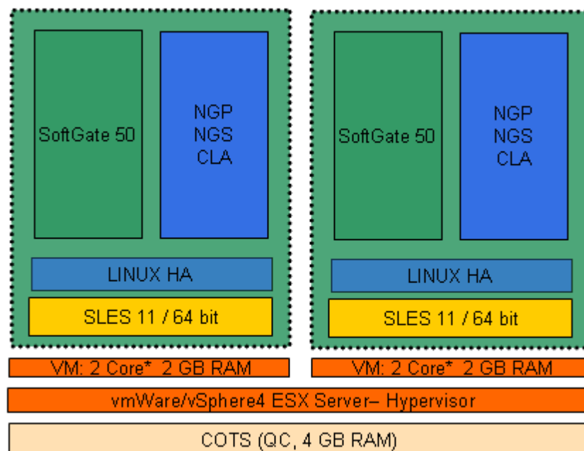
Figure 31: Virtualized OpenScape 4000 SoftGates
