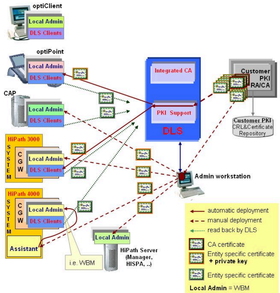
Figure 55: Certificate generation and deployment for secure WBM access
