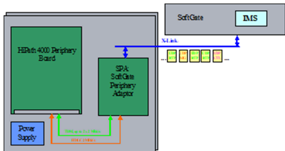
Figure 21: OpenScope Access Module with OpenScope 4000 Softgate connection
