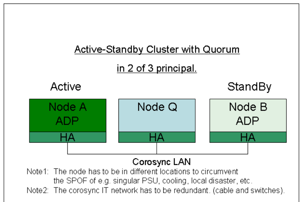
Figure 9: Quorum node configuration
