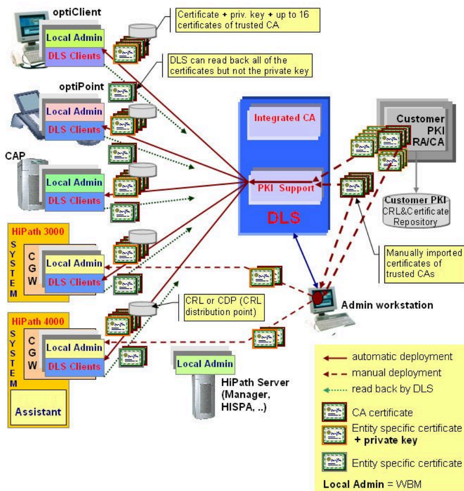
Figure 56: Certificate generation and deployment for SPE: customer PKI
