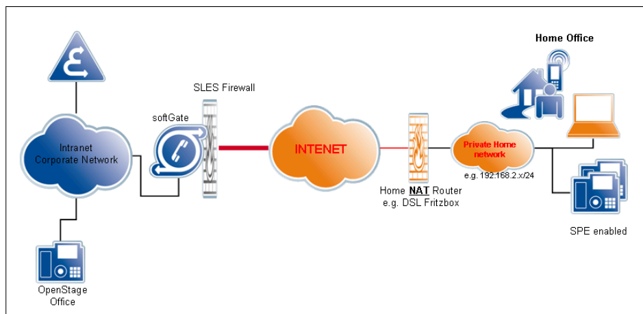
Figure 36: Secure Remote Subscriber
