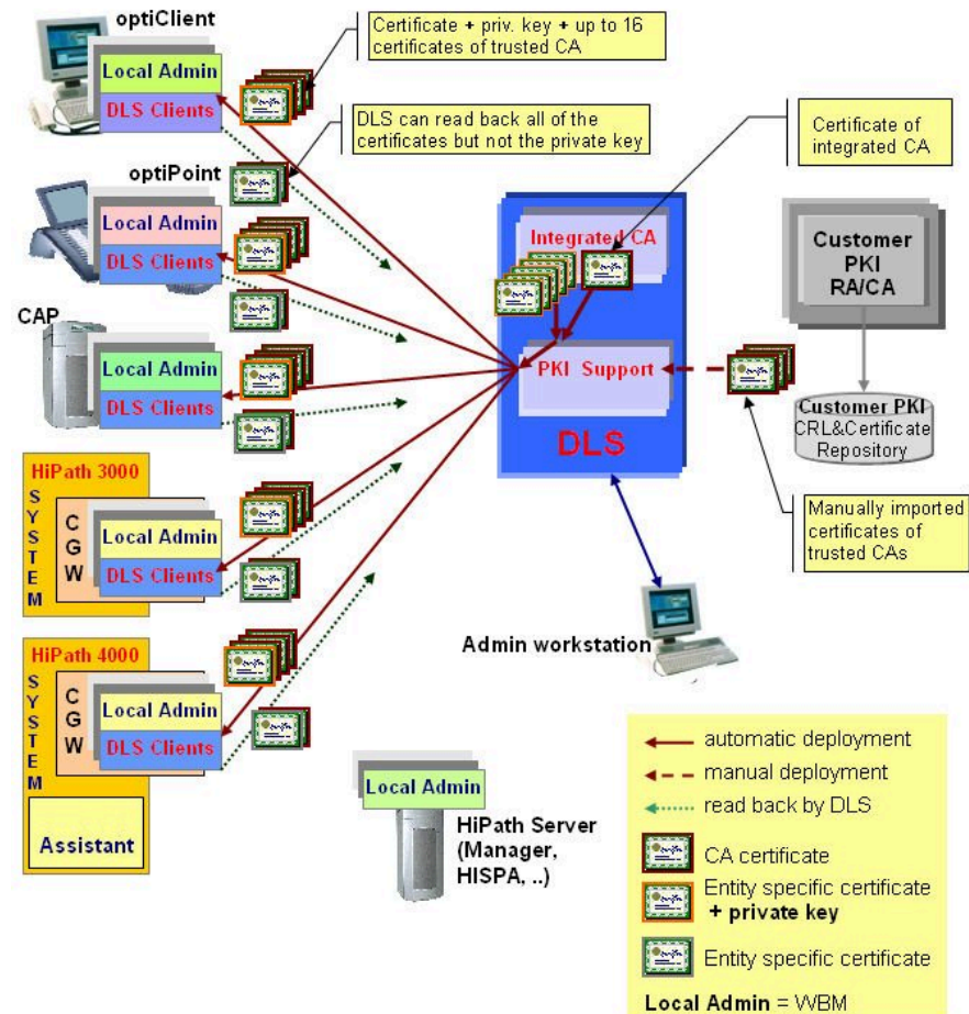
Figure 57: Certificate generation and deployment for SPE: DLS integrated CA
