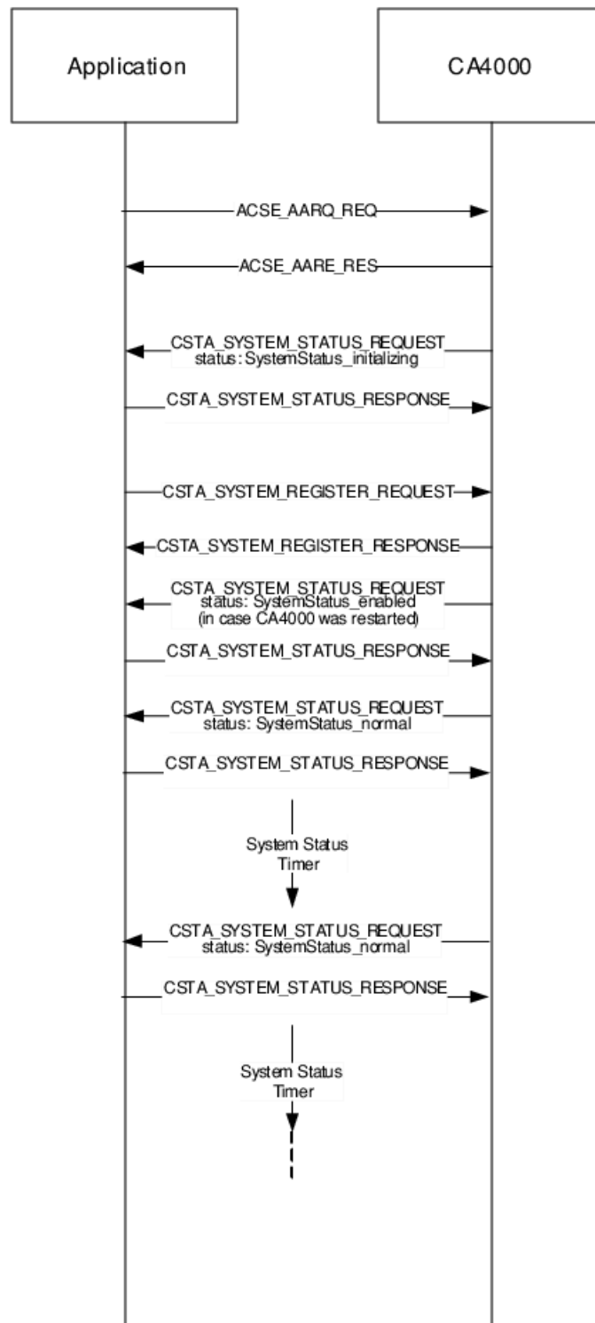
Figure 2: Successful connection
