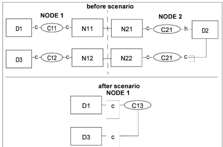
Figure 98: Route optimization
