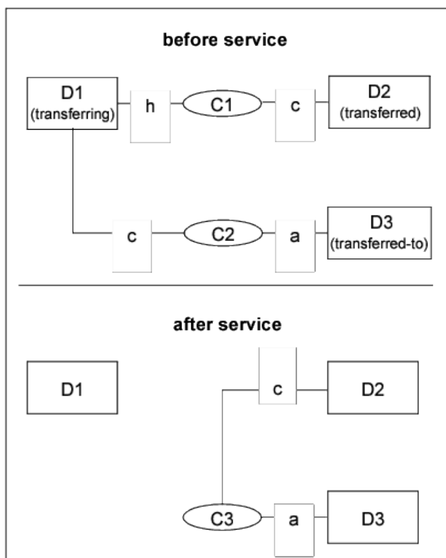
Figure 55: Blind transfer
