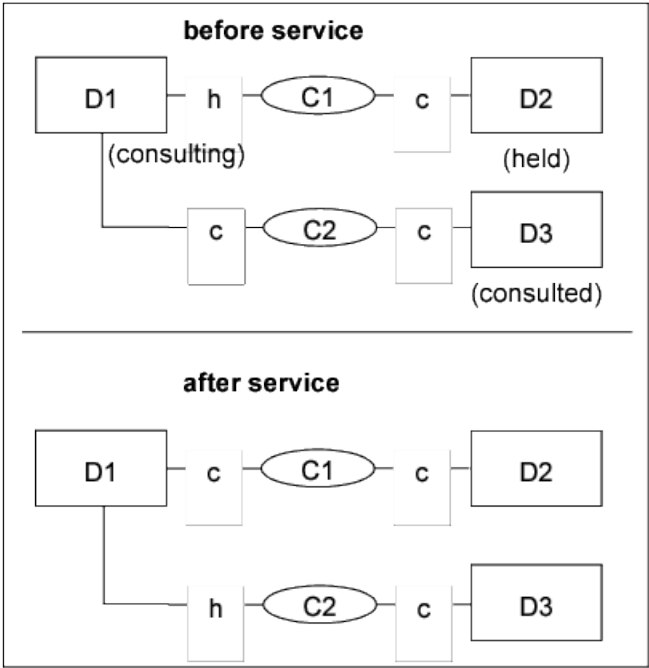
Figure 51: Alternate call
