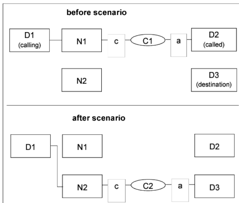
Figure 39: Deflect call with rerpouting enabled
