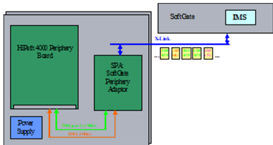
Figure 40: OpenScope Access Module with 4000 Softgate / Access 500
