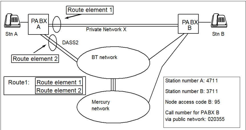
Figure 70: Example for out dial rules
