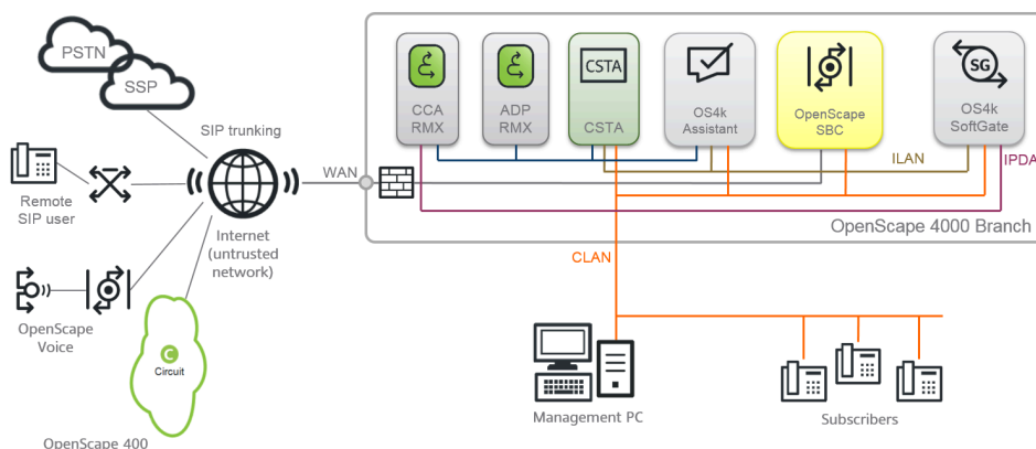
Figure 61: SBC hosted on OpenScape 4000 Branch
