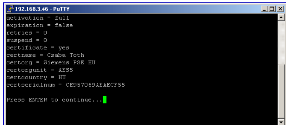
Figure 2: Print current settings
