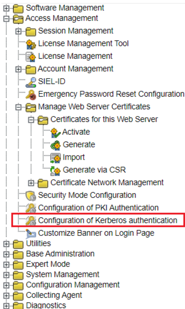
Figure 4: Access to the Configuration of Kerberos Authentication
