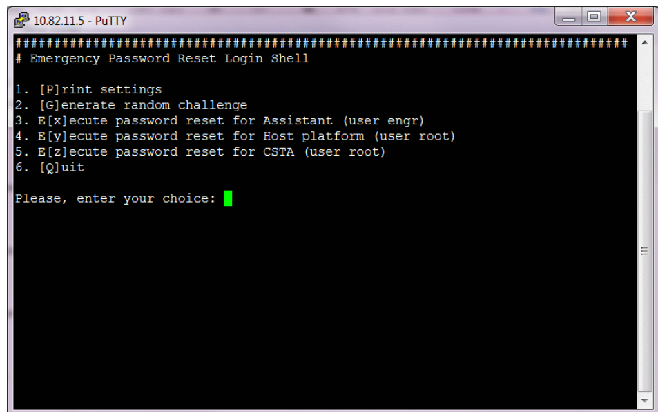
Figure 1: EPR login shell, initial menu
