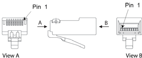
Fig. 25 Pin-nummering, RJ45 connector
