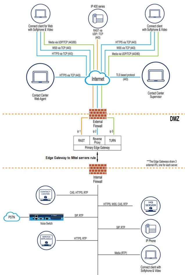
Figure 2: Network Architecture
