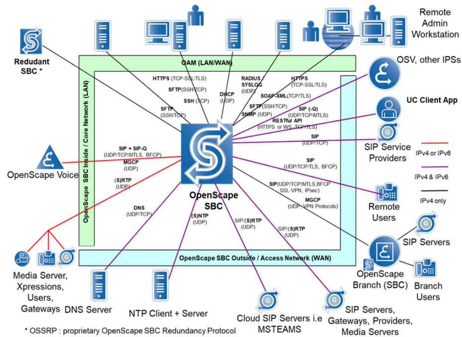
Figure: OpenScape SBC Interfaces and Protocols
