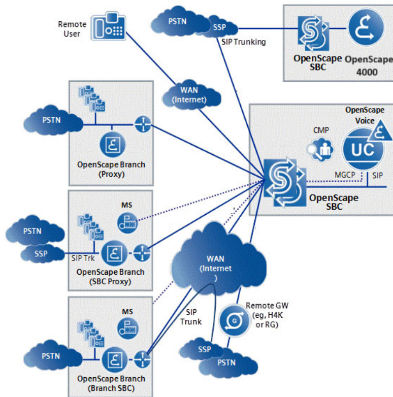
Figure: OpenScape SBC Single Arm Deployment for MS TEAMS Overview
