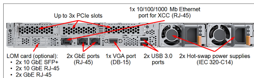
Figure 4: Lenovo SR530, Rear view
