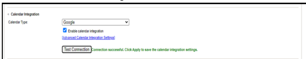
Figure 26: Calendar Integration
