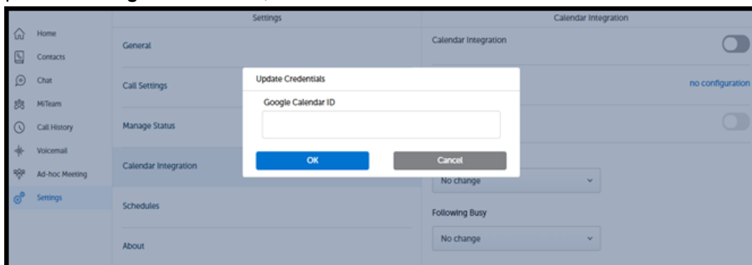
Figure 27: Update Credentials
