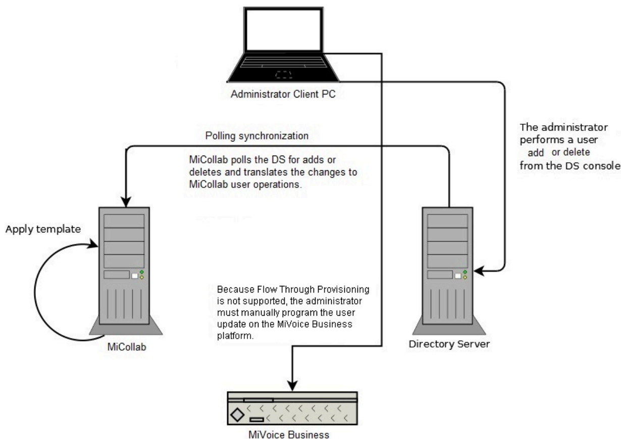
Figure 10: MiCollab and MiVoice Business (s) without Single Point Provisioning
