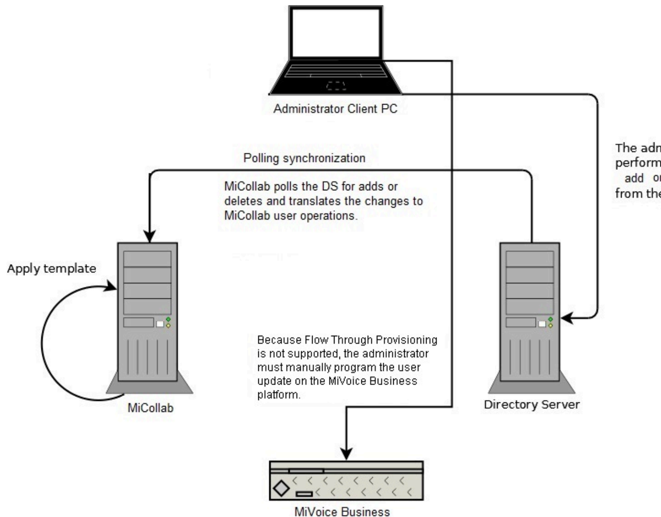
MiCollab and MiVoice Business (s) without Single Point Provisioning
