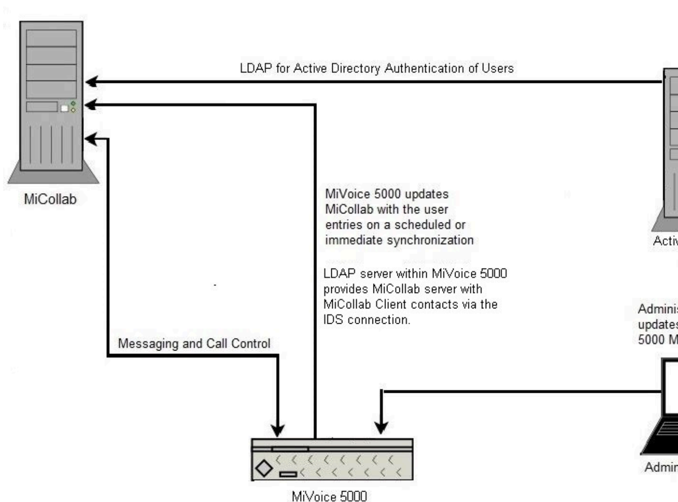
Figure 5: Single MiCollab Server and a Single MiVoice 5000
