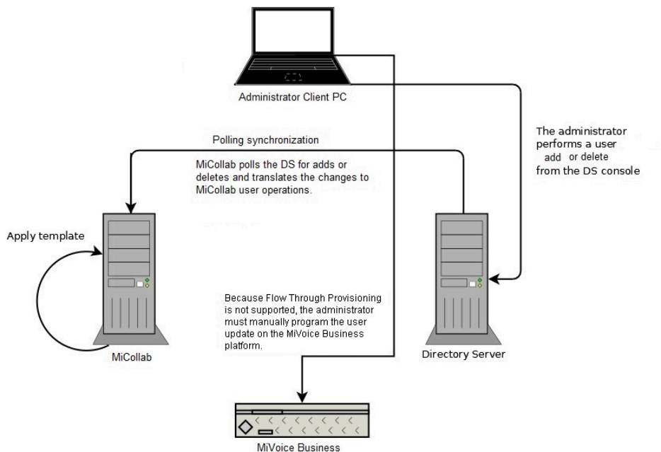
MiCollab and MiVoice Business (s) without Single Point Provisioning
