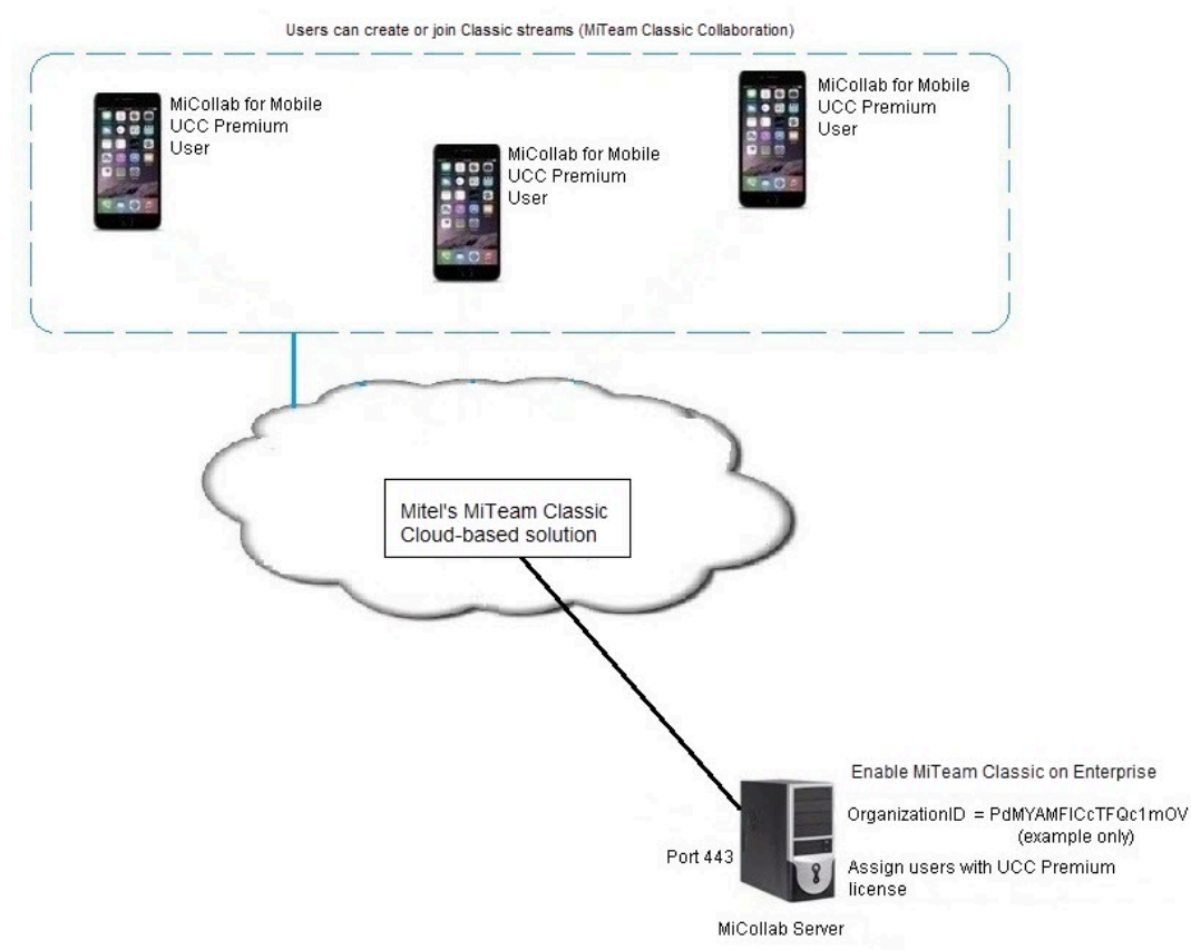
Figure 1: MiTeam Classic – Enterprise Configuration (Non-Peered)
