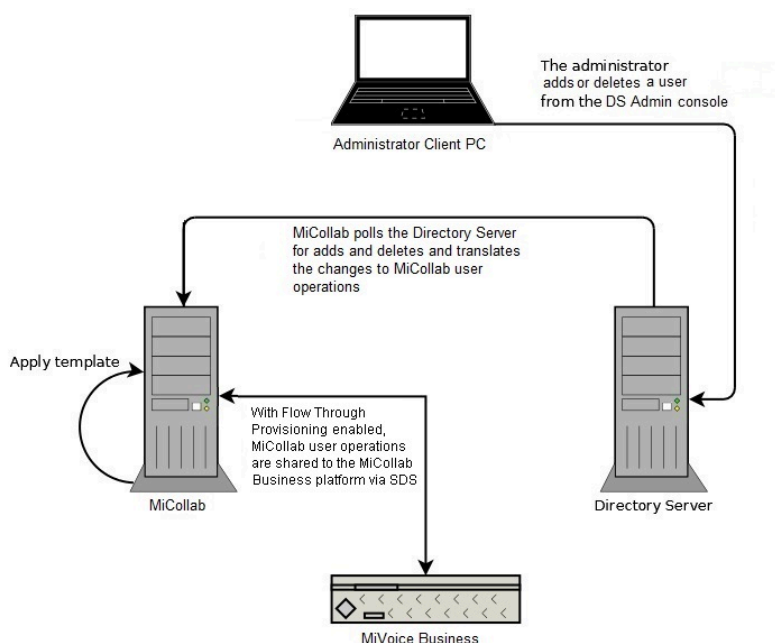
MiCollab and MiVoice Business (s) with Flow Through Provisioning
