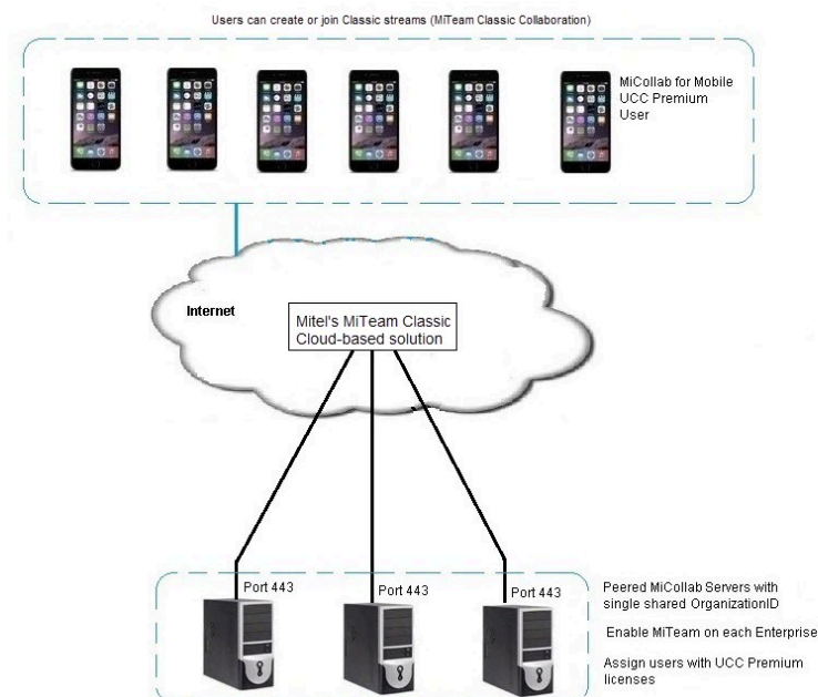
Figure 6: MiTeam Classic – Peered Enterprise Configuration
